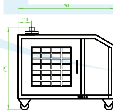
External drawing of the Rigid line 1 5/8"
